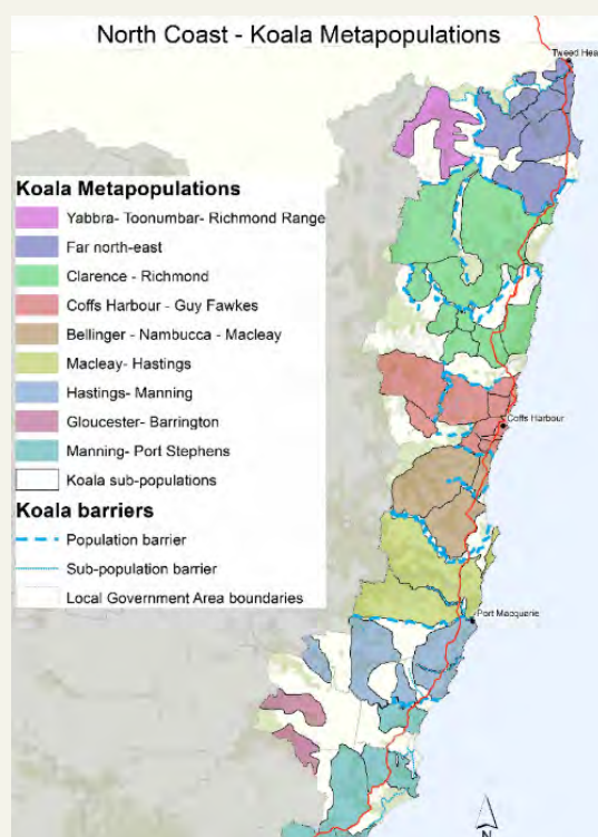
Figure 13. Populations in the GKNP
