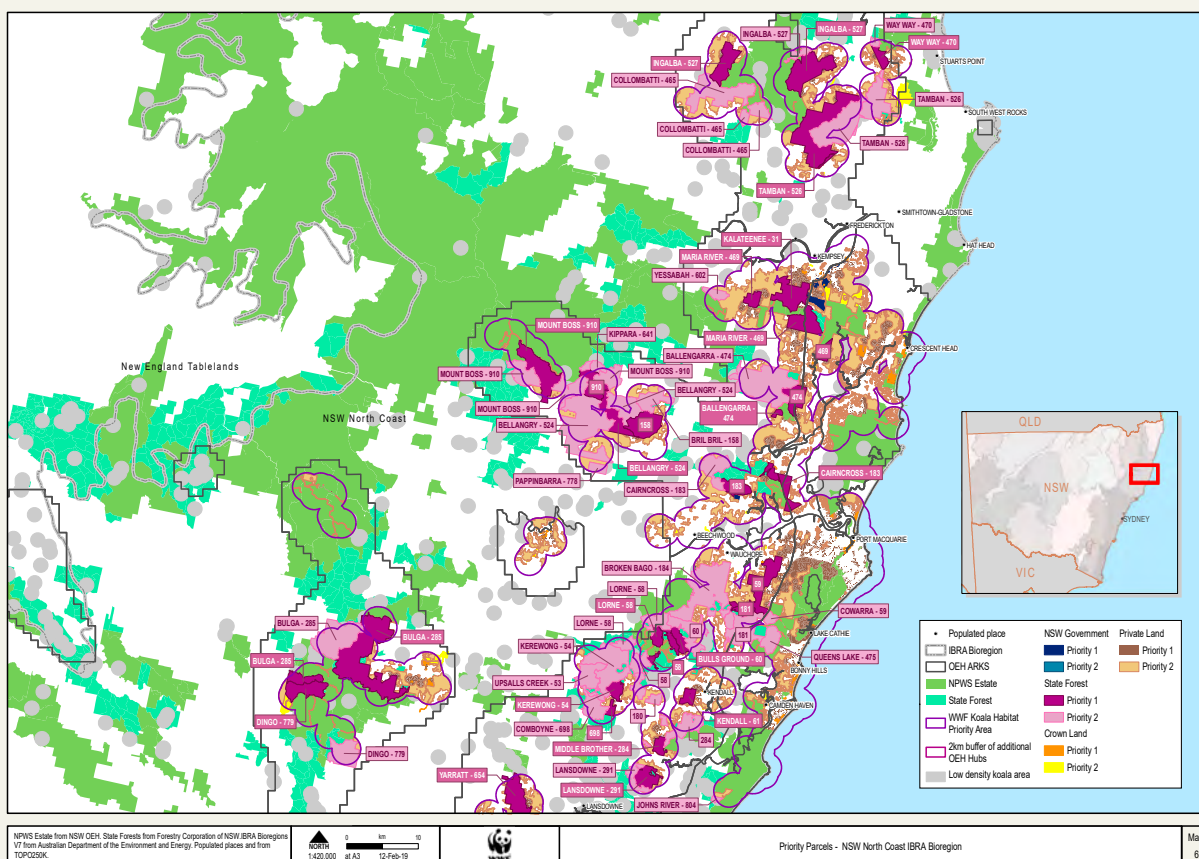
Map 6. NSW North Coast IBRA Bioregion (central)
