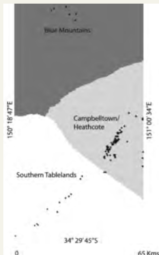
Figure 2. Populations of koalas in southwestern Sydney. Each dot represents genetic sampling location. (from Lee et al. 2010).
