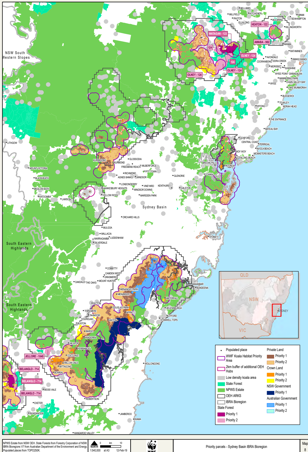
Map 8. Sydney Basin IBRA Bioregion
