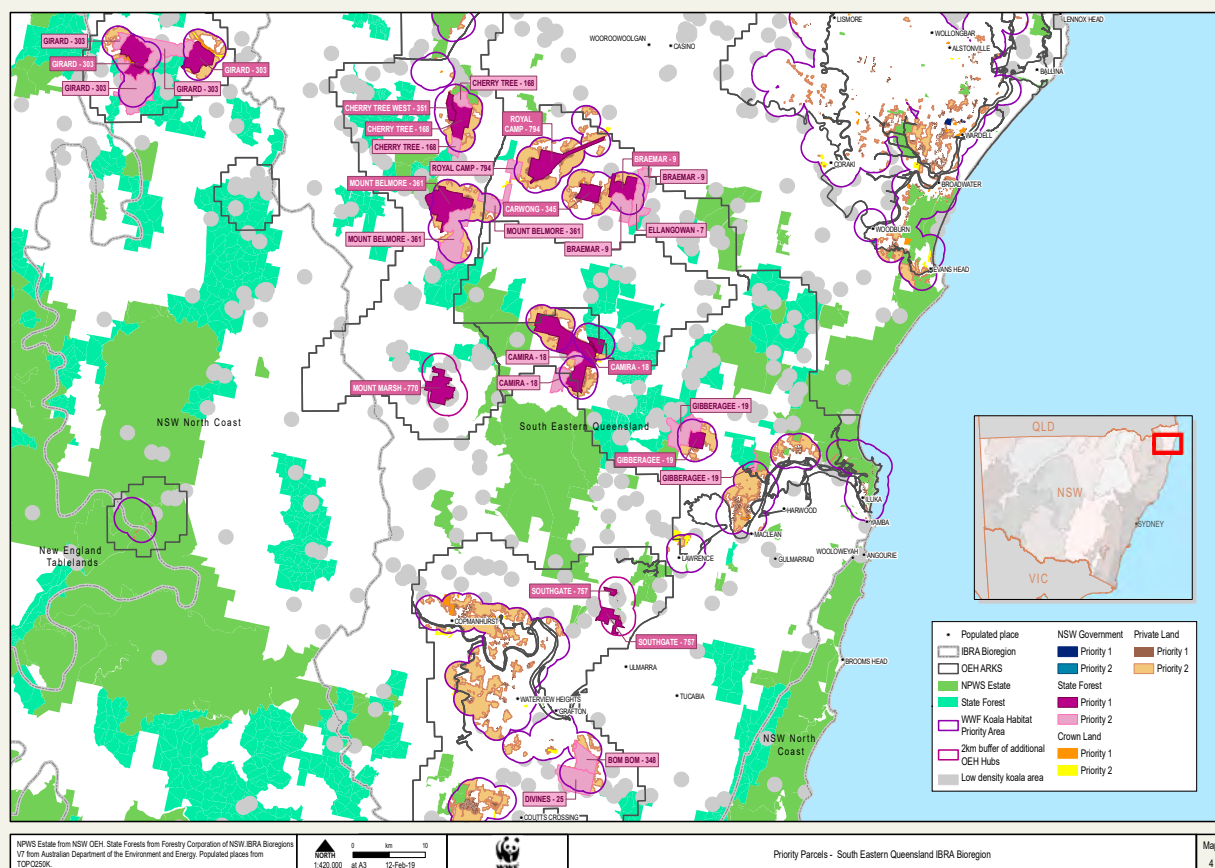
Map 4. Priority Parcels - South East Queensland IBRA Bioregion (southern)
