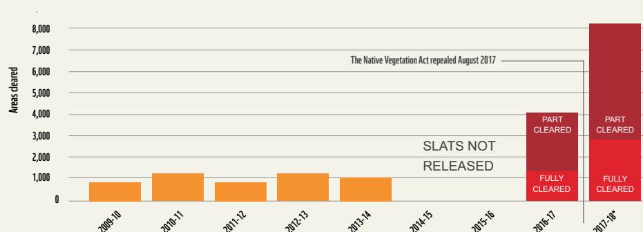
Figure 4. Recent land clearing rates in the Moree and Collarenebri area of North-west NSW (from WWF-Australia and NCC, 2018). The chart shows the area of land cleared each year in the study 22,000 km 2 area according to NSW SLATS from 2009 to 2014, and fully or partly cleared according to this analysis for 2016-18. * see Figure 2, WWF-Australia and NCC (2018) for details.
