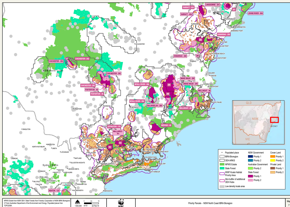
Map 7. NSW North Coast IBRA Bioregion (southern)
