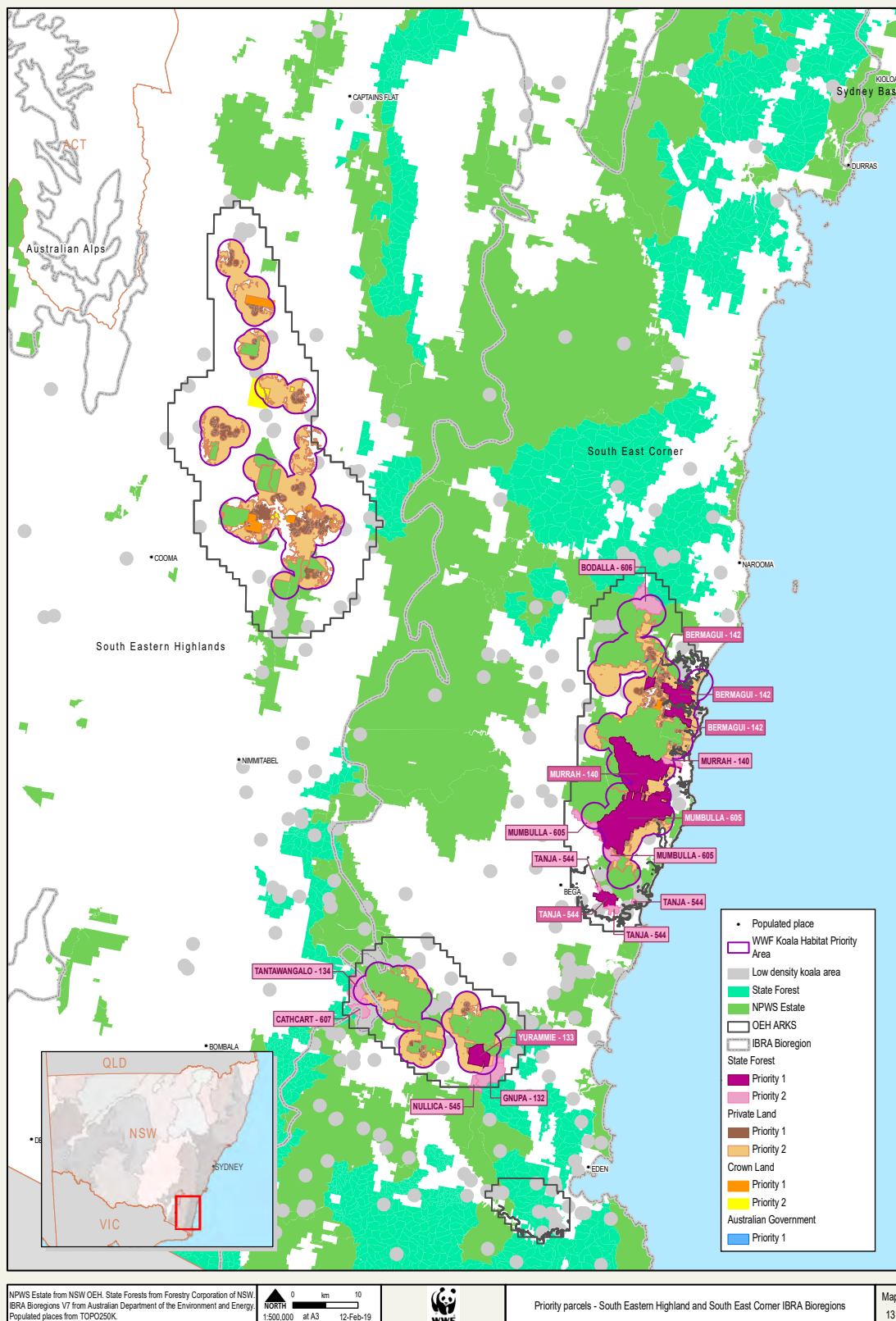
Map 13. South Eastern Highlands and South East Corner IBRA Bioregions
