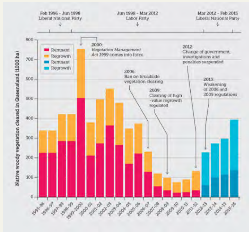
Figure 5. Land clearing statistics for Queensland 1995-2016 (from Stefan and Dean 2018). The chart depicts a history of vegetation clearing in Queensland showing increased clearing rates in blue. Remnant vegetation is woody vegetation that has not been previously allowed to regrow to maturity after earlier clearing. Regrowth is woody vegetation that has been cleared and is in the process of regrowing but has not yet reached maturity.
