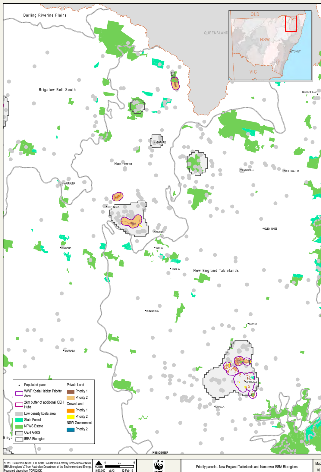
Map 10. New England Tablelands and Nandewar IBRA Bioregions
