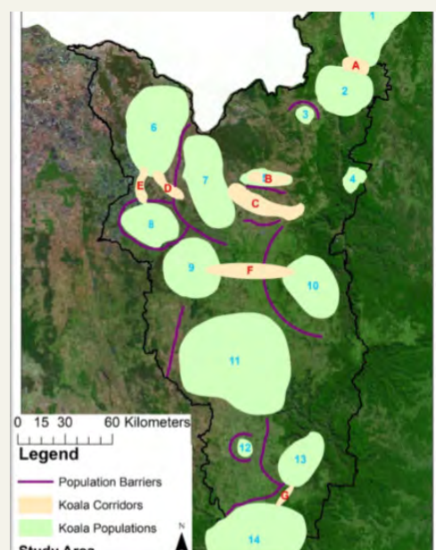
Figure 15. Key corridors and populations (Envirolink 2016)
