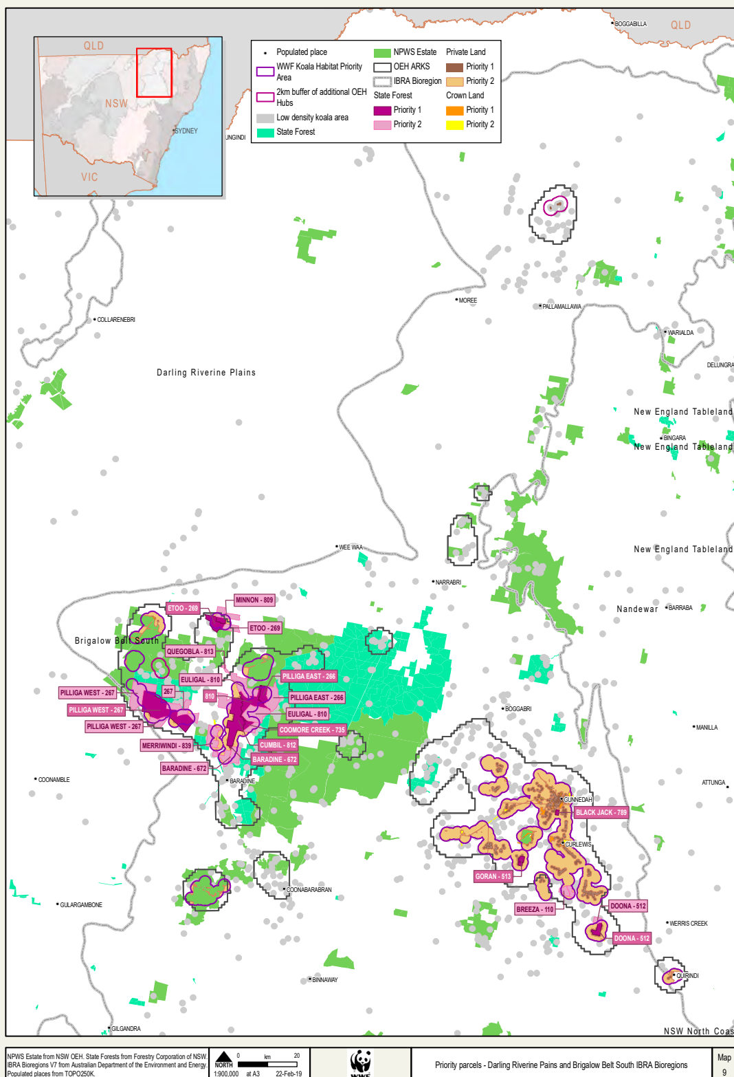
Map 9. Darling Riverine Plains and Brigalow Belt South IBRA Bioregions
