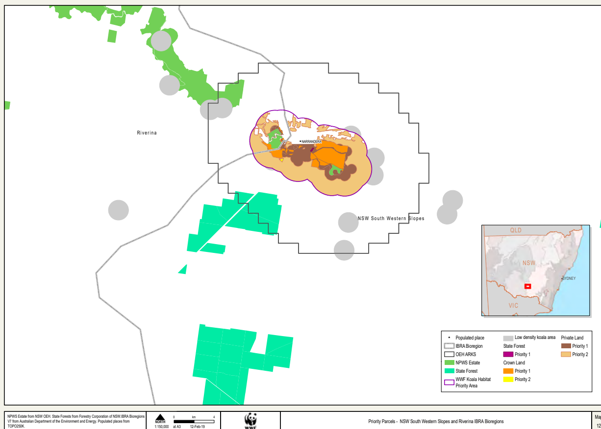
Map 12. NSW South Western Slopes and Riverina IBRA Bioregions
