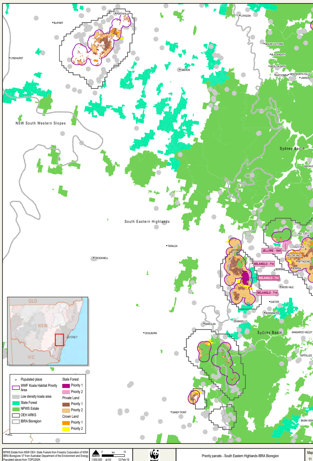
Map 11. South Eastern Highlands IBRA Bioregion
