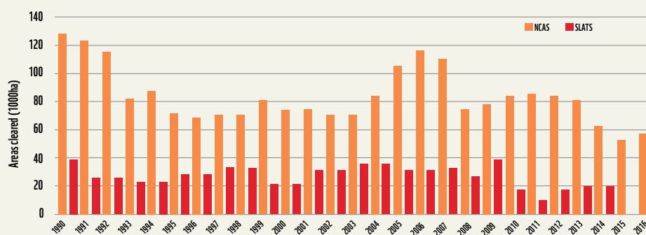
Figure 3. Rates of land clearing in NSW (1990-2016) (from WWF-Australia and NCC 2018). The chart shows a comparison of total land clearing in NSW as estimated by the NSW Government’s Statewide Land and Tree Study (SLATS, excluding fires and plantation harvest) (red bars) and as estimated by the Australian Government’s National Carbon Accounting System (NCAS) (orange bars).
