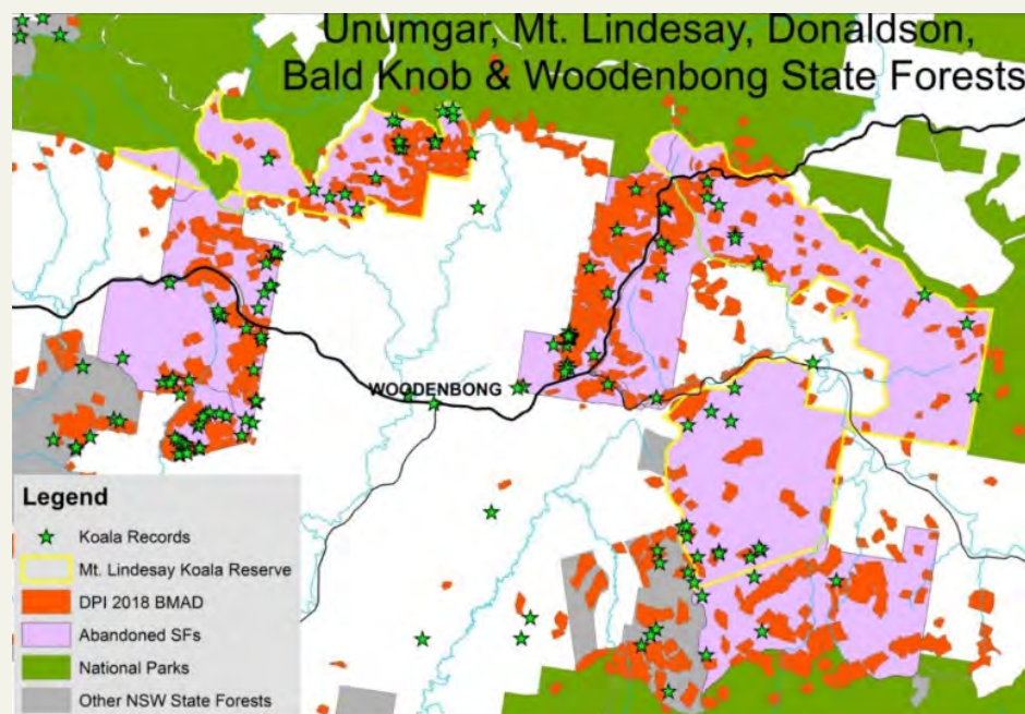
Figure 12. Koala records in relation to Bell Miner-Associated Dieback as under-mapped by DPI-Forestry (Silver and Carnegie 2017). Areas of state forest abandoned for timber production (pink areas) and the proposed Mt. Lindesay Koala Reserve (see yellow outline). Note the high correlation of koala records with dieback areas, emphasising the urgent need for protection and rehabilitation of these important areas.
